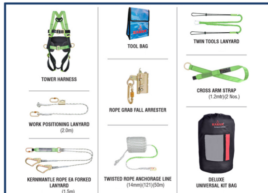
TOWER KIT
